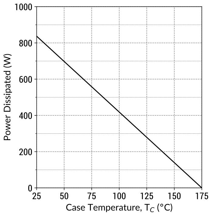
Figure 3: Power Derating Curves
