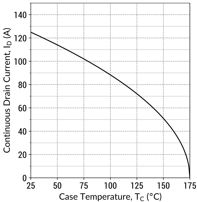
Figure 15: Current De-rating Curve
